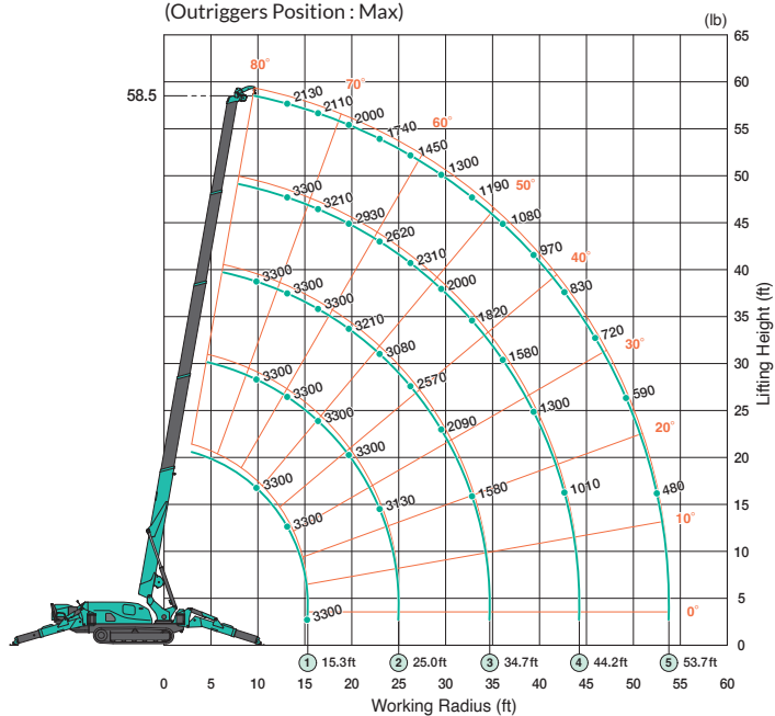
3,300lb Searcher Hook Offset Position : SH3 (Outriggers Position : Max)
