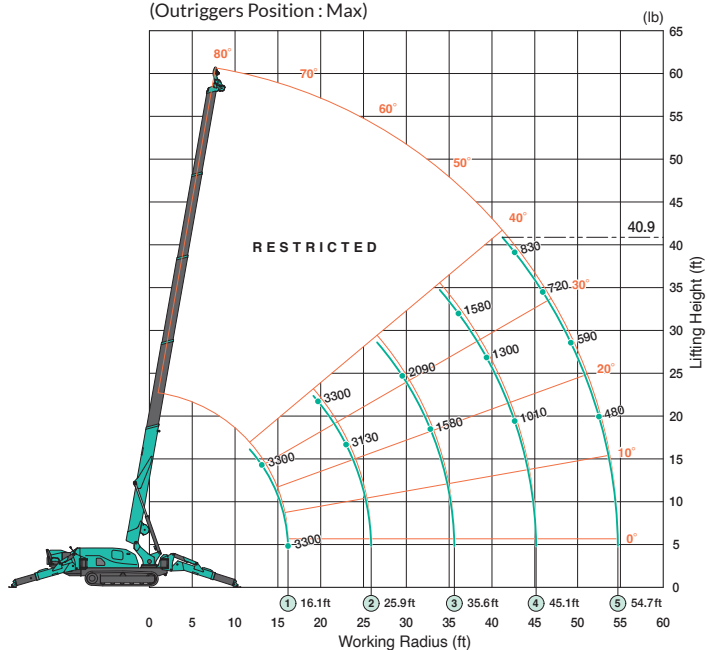
3,300lb Searcher Hook Offset Position : SH1 (Outriggers Position : Max)
