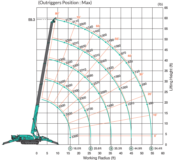
3,300lb Searcher Hook Offset Position : SH2 (Outriggers Position : Max)
